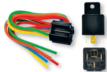
64-102P 12V, 5 Pin, 30A, SPDT Relay Kit with Mounting Bracket
