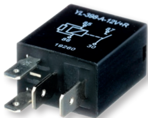
64-110P 12V, 4 Pin, 30A, Micro Relay
