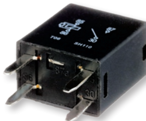
64-108P 12V, 4 Pin, 30A, Micro Relay
