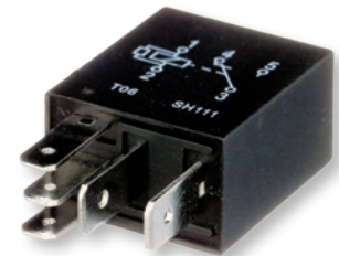
64-106P 12V, 5 Pin, 20A, Micro Relay, Multi-Function, A/C Compressor Clutch
